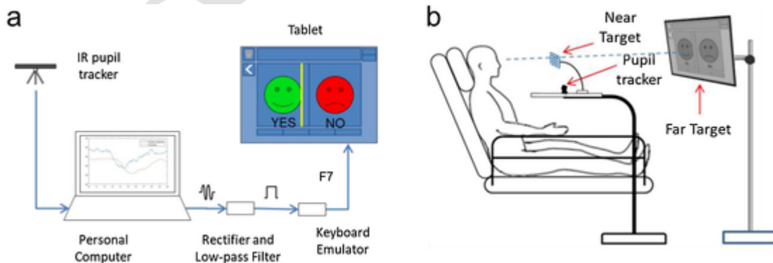
Fig. 1. a) Functional scheme of the communication prototype: the personal computer, fed by the eye-tracker, detects the pupil constriction and generates a «beep» on the headphones output; this signal is transformed into a trigger signal for the scanning selection operated on the tablet. b) Experimental set-up: note the alignment of the semi-transparent near target and the far target (tablet), with the subject's gaze.
