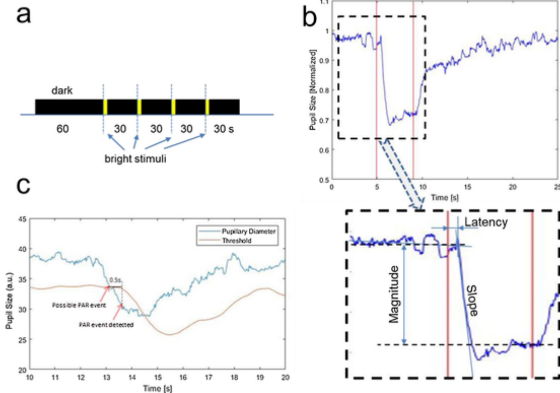
Fig. 2. Methodological illustrations. a) Pupil light reflex assessment protocol. Four bright stimuli, lasting 4 s are delivered during an otherwise completely dark visual field.; b) Pupil light reflex. The pupil size is normalized to the basal level (dark condition). The red vertical lines indicate start and end of the 4-s lasting light stimulus. The tracing represents the average of 4 responses. The magnification below is used to show the parameters extracted from the curve; c) Detection of the pupil accommodative response. The threshold level (brown) is obtained from the pupil size signal smoothed by a moving average (0.8-s size), delayed by 0.8 s, and attenuated by 10 %. A valid pupil constriction is detected whenever the pupil size remains below threshold for at least 0.5 s.
