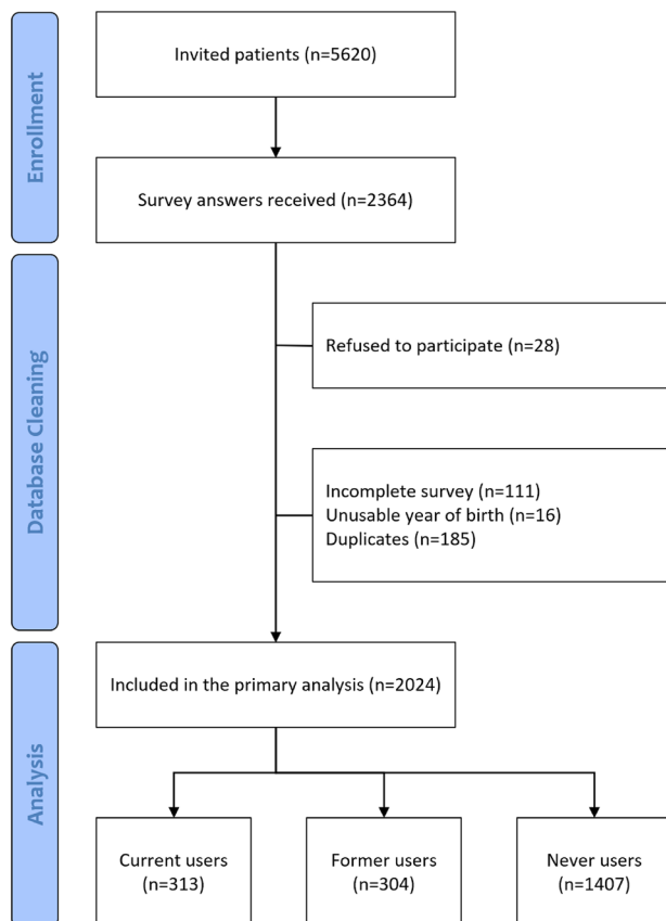
Fig. 1 Study flow-diagram
