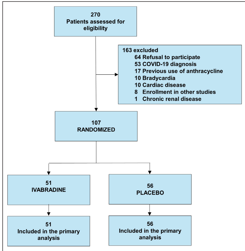
Figure 2. Study flowchart.
