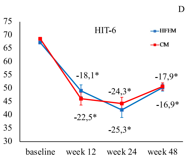
Fig. 2 d Headache Impact Test-6 (HIT-6) score from baseline to week 48 in patients affected by high-frequency episodic migraine (HFEM, n=49 ) or chronic migraine (CM, n=81 )
